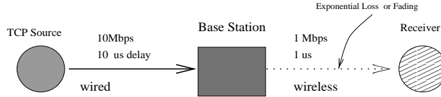
Figure 8. Topology for Experiments 1 - 3
