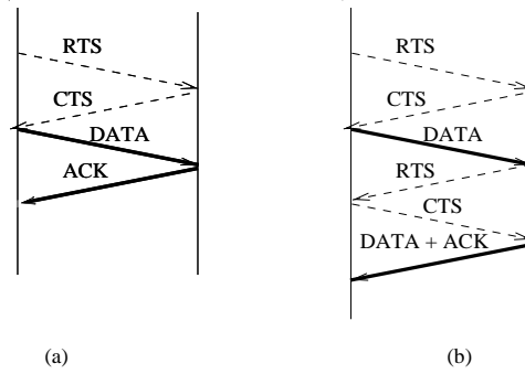
Figure 4. (a) MAC Acceleration: FAMA transmits TULIP data packet and returns ACK without another RTS/CTS exchange. Returning TULIP ACK may contain a TCP ACK. (b) FAMA exchange with large ACK packet (encapsulated data packet) requires another RTS/CTS exchange.
